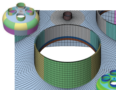
Hexahedral Mesh
